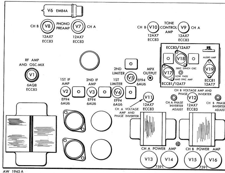
FIGURE 2. Tube layout.
